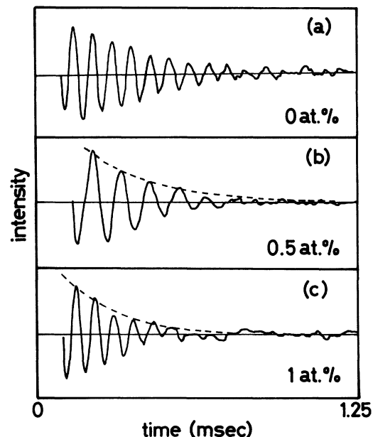
FIG. 1. Solid lines are FID's of 89 Y NMR in the magnetically dilute alloys Gd x Y 1-x Ba 2 Cu 3 O 7-δ at 100 K. The beat is due to a difference between the Larmor and the rf frequency. Necessary information is the decay time constant of the intensity and not the presence of the beat. Dashed lines are calculated decay curves from the dipolar local fields. (a) x=0 , (b) x=0.005 , and (c) x=0.01 .
